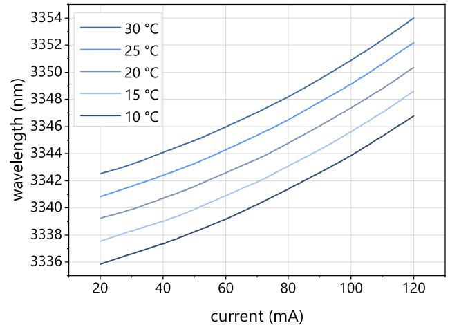
Typical mode hop free tuning of a nanoplus DFB ICL at 3345 nm by current and temperature
