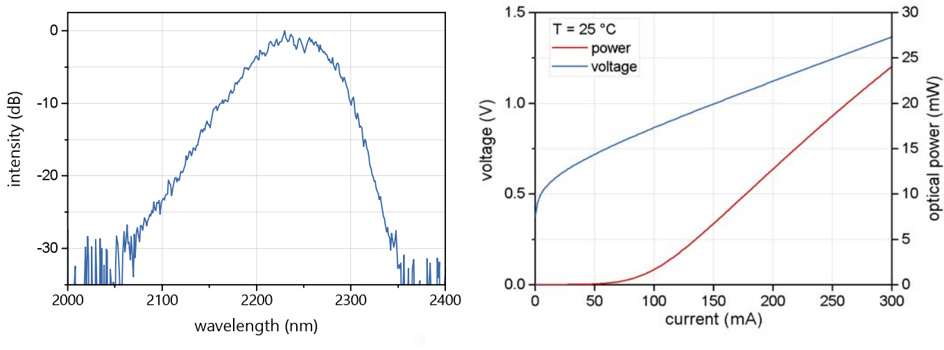
Typical room temperature cw spectrum of a nanoplus SLD at 2245 nm
