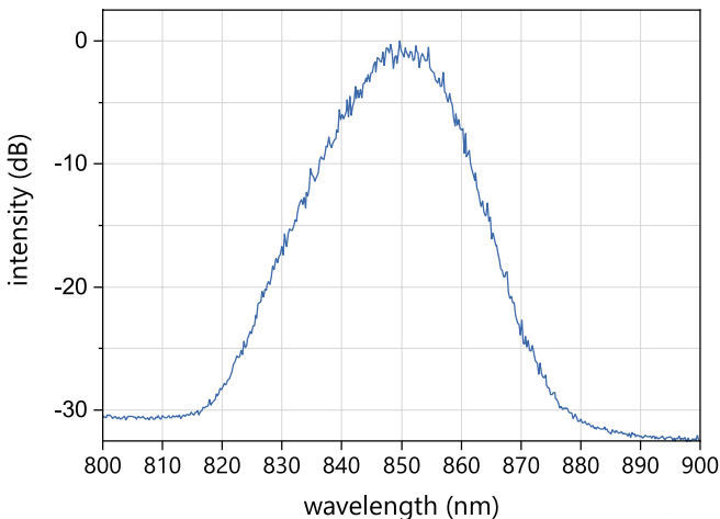
Typical room temperature cw spectrum of a nanoplus SLD at 850 nm
