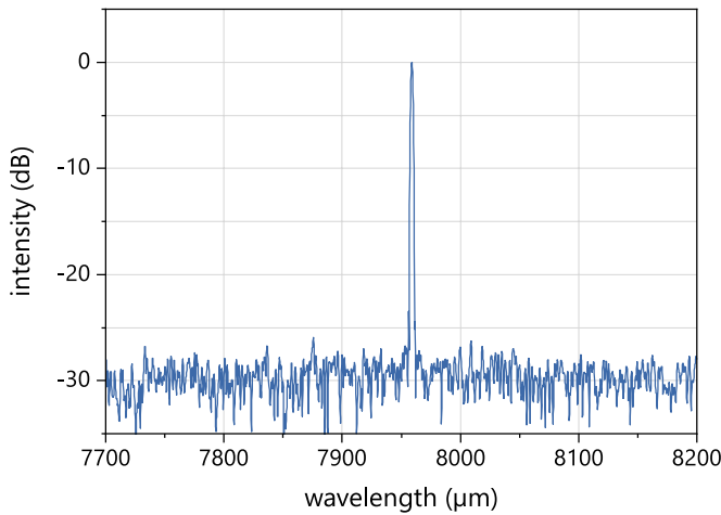
Typical room temperature cw spectrum of a nanoplus DFB ICL at 7970 nm
