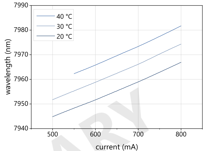
Typical mode hop free tuning of a nanoplus DFB ICL at 7970 nm by current and temperature
