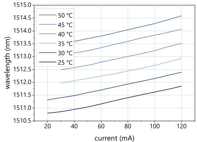
Typical mode hop free tuning of a nanoplus DFB laser at 1512.2 nm by current and temperature
