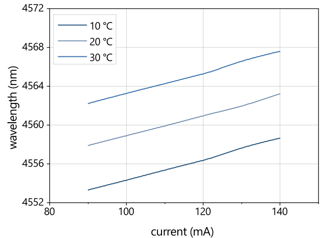
Typical mode hop free tuning of a nanoplus DFB ICL at 4565 nm by current and temperature
