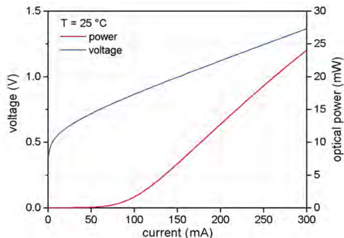
Typical PI and VI curve of a nanoplus SLD at 2245 nm
