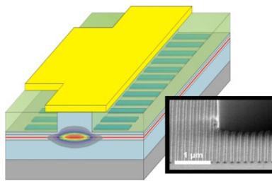
Schematic of nanoplus DFB laser
