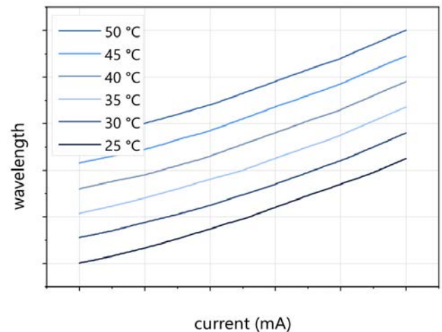
Typical mode-hop-free tuning of a nanoplus DFB laser by current and temperature
