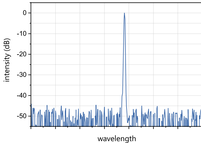
Typical cw spectrum of a nanoplus DFB laser at room temperature
